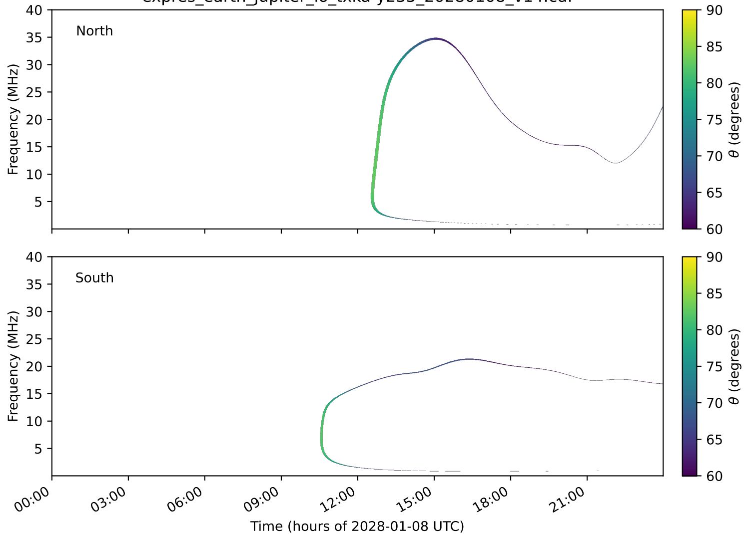
expres_earth_jupiter_io_txka-y235_20280108_v14.cdf
