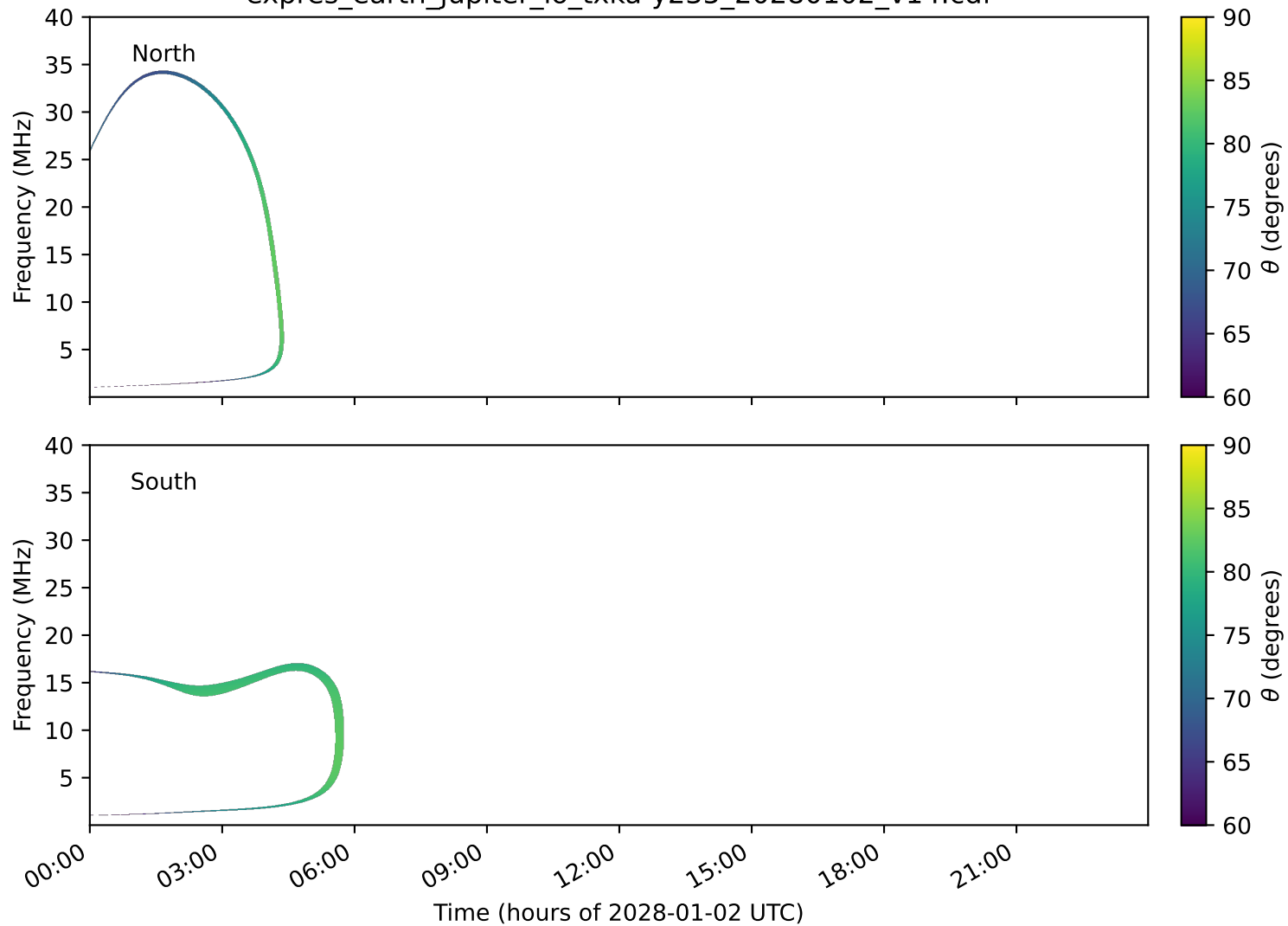
expres_earth_jupiter_io_txka-y235_20280102_v14.cdf
