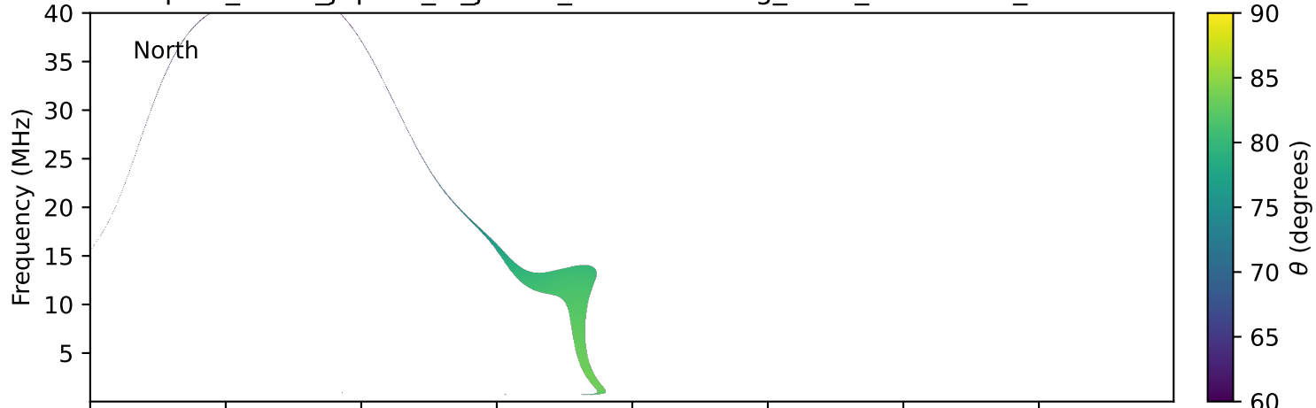
expres_earth_jupiter_io_jrm33_lossc-wid1deg_3kev_20280130_v11.cdf
