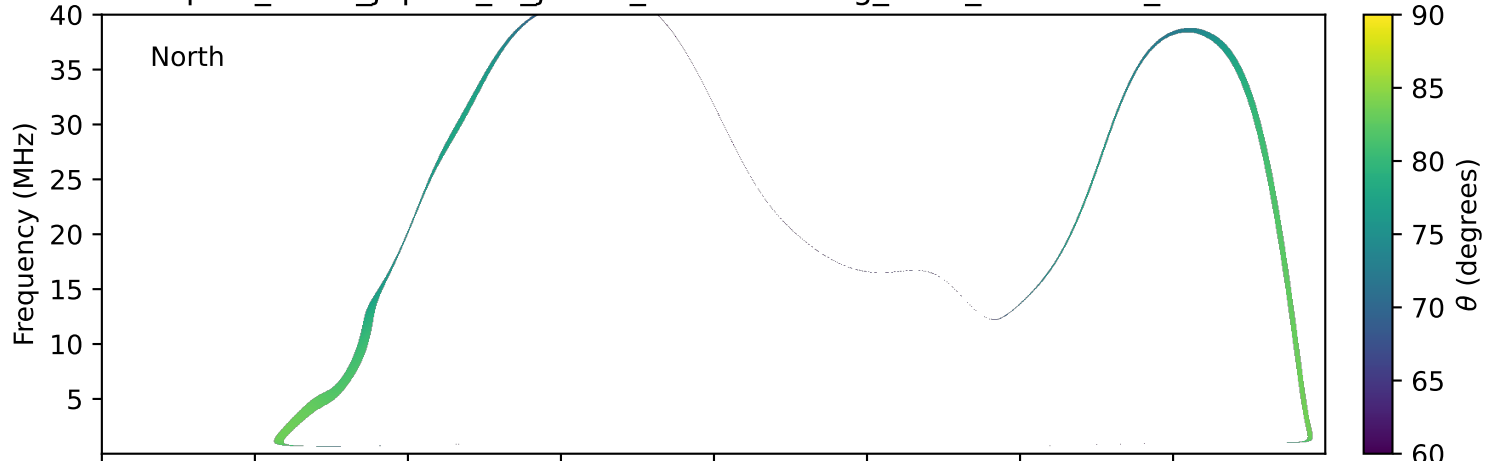
expres_earth_jupiter_io_jrm33_lossc-wid1deg_3kev_20280126_v11.cdf
