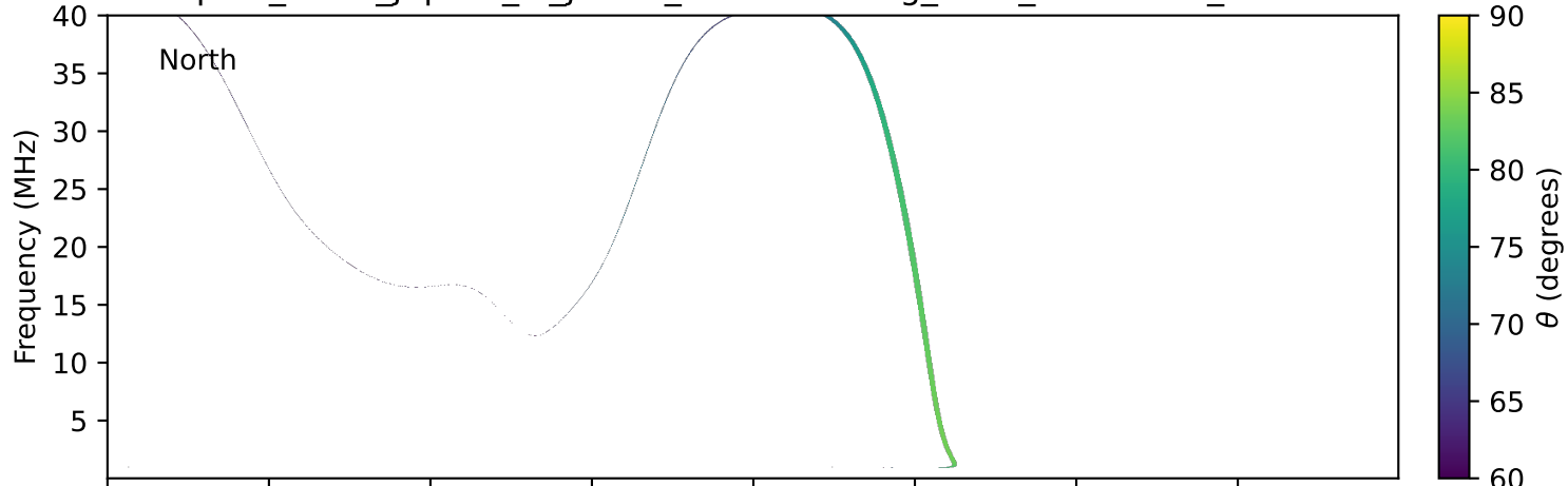
expres_earth_jupiter_io_jrm33_lossc-wid1deg_3kev_20280121_v11.cdf
