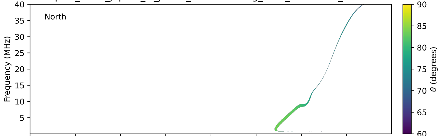
expres_earth_jupiter_io_jrm33_lossc-wid1deg_3kev_20280106_v11.cdf
