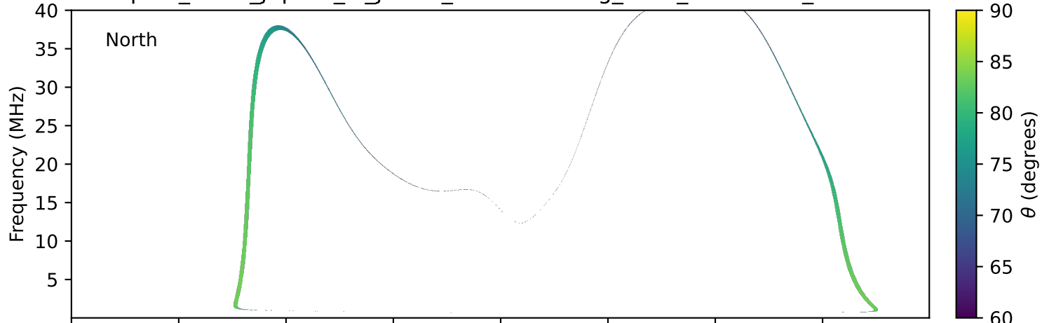
expres_earth_jupiter_io_jrm33_lossc-wid1deg_3kev_20280103_v11.cdf
