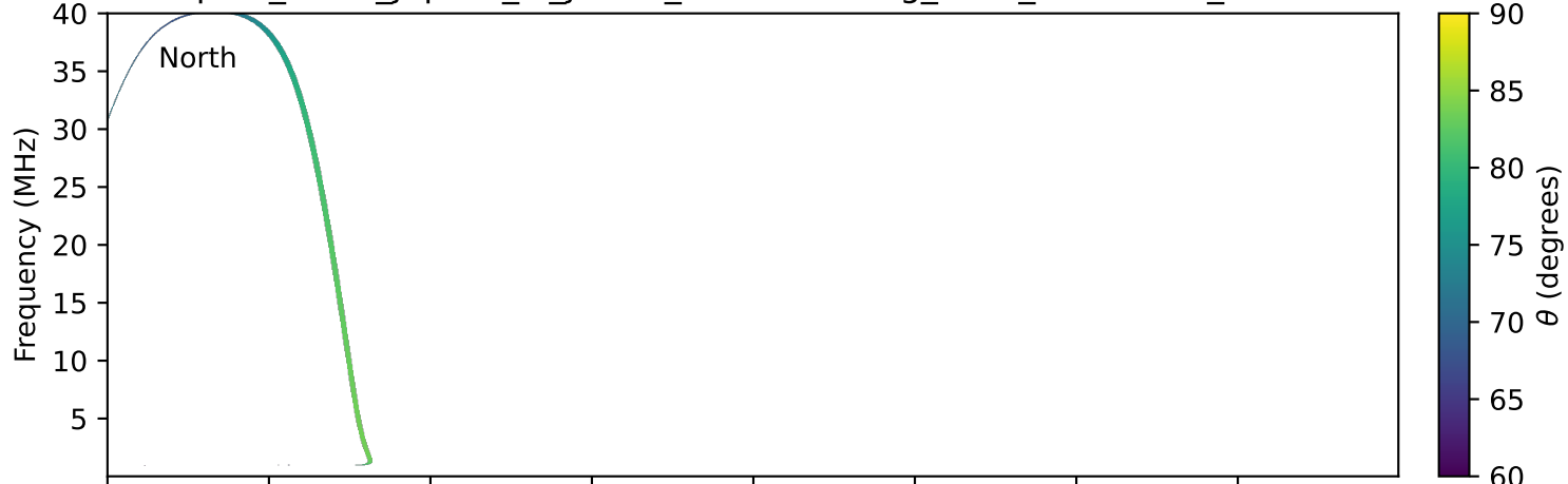
expres_earth_jupiter_io_jrm33_lossc-wid1deg_3kev_20280102_v11.cdf
