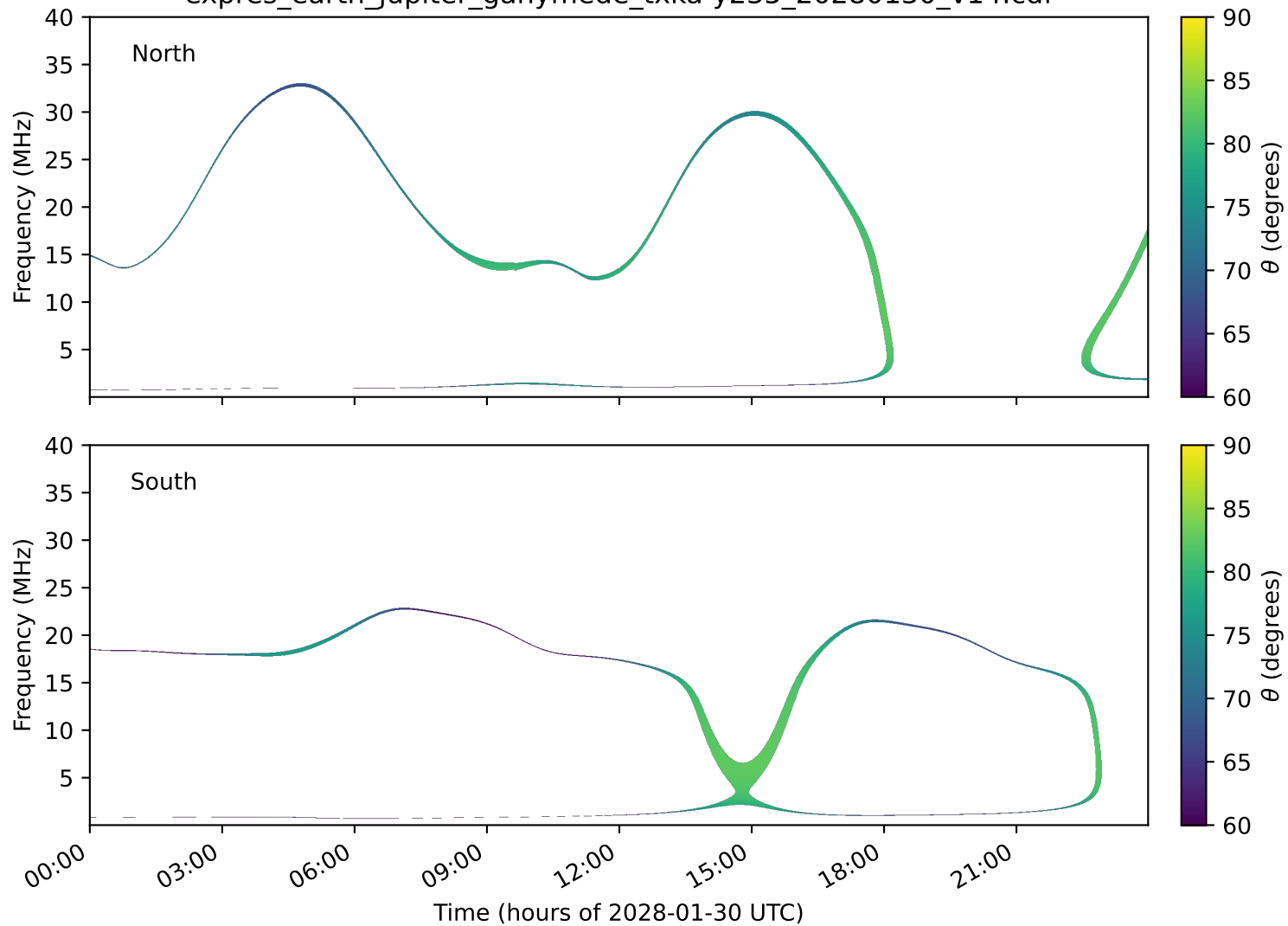
expres_earth_jupiter_ganymede_txka-y235_20280130_v14.cdf
