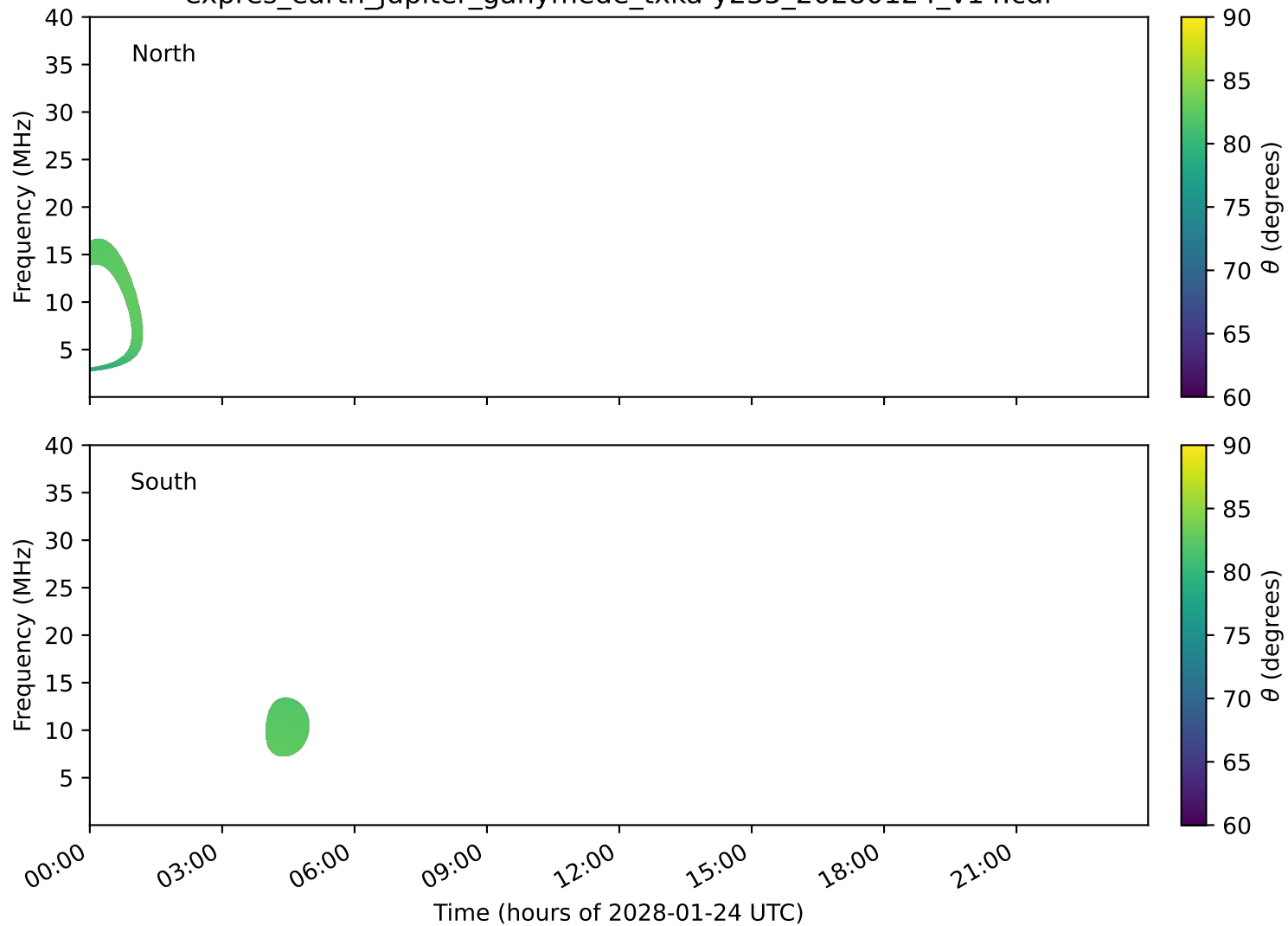
expres_earth_jupiter_ganymede_txka-y235_20280124_v14.cdf
