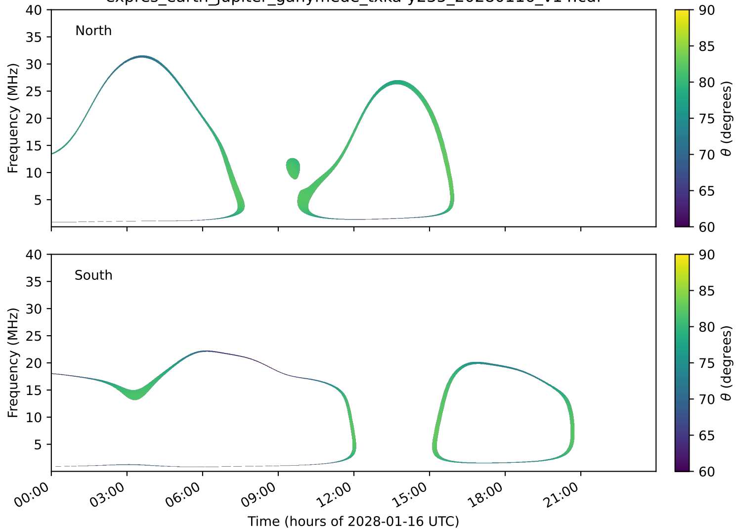
expres_earth_jupiter_ganymede_txka-y235_20280116_v14.cdf
