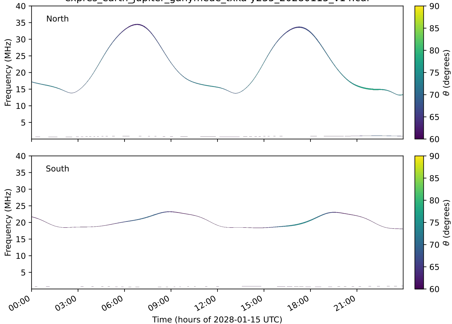
expres_earth_jupiter_ganymede_txka-y235_20280115_v14.cdf
