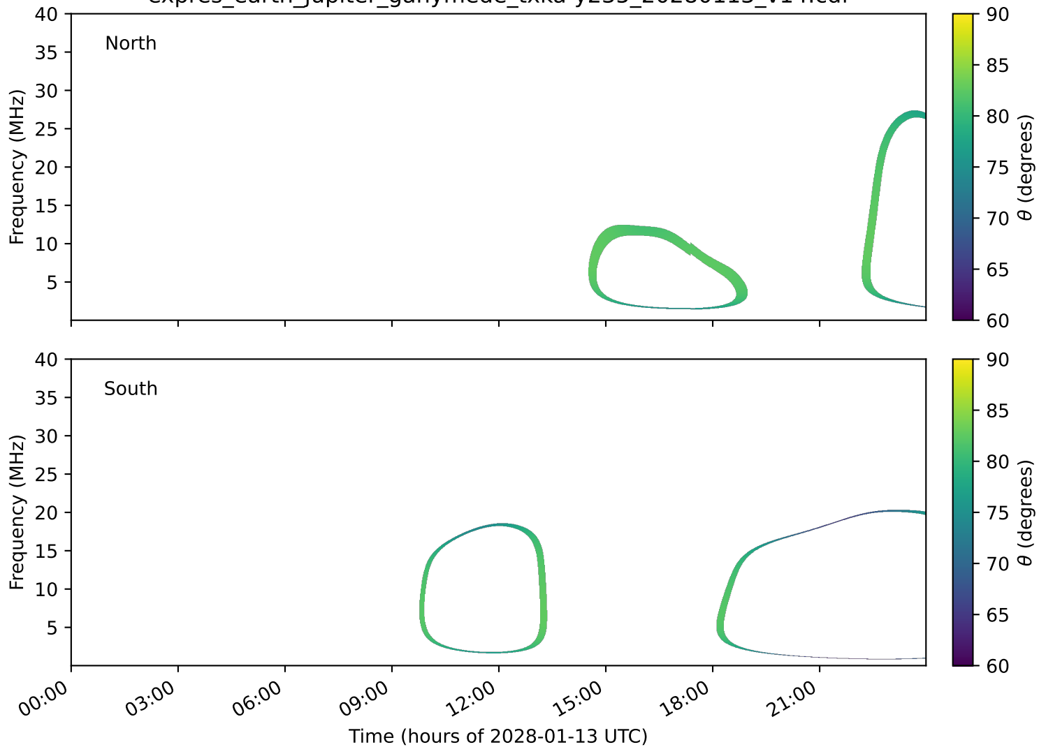
expres_earth_jupiter_ganymede_txka-y235_20280113_v14.cdf
