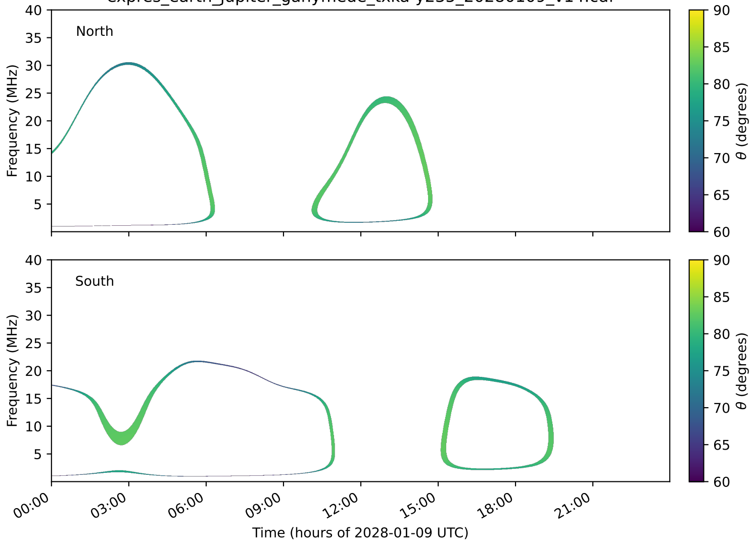
expres_earth_jupiter_ganymede_txka-y235_20280109_v14.cdf
