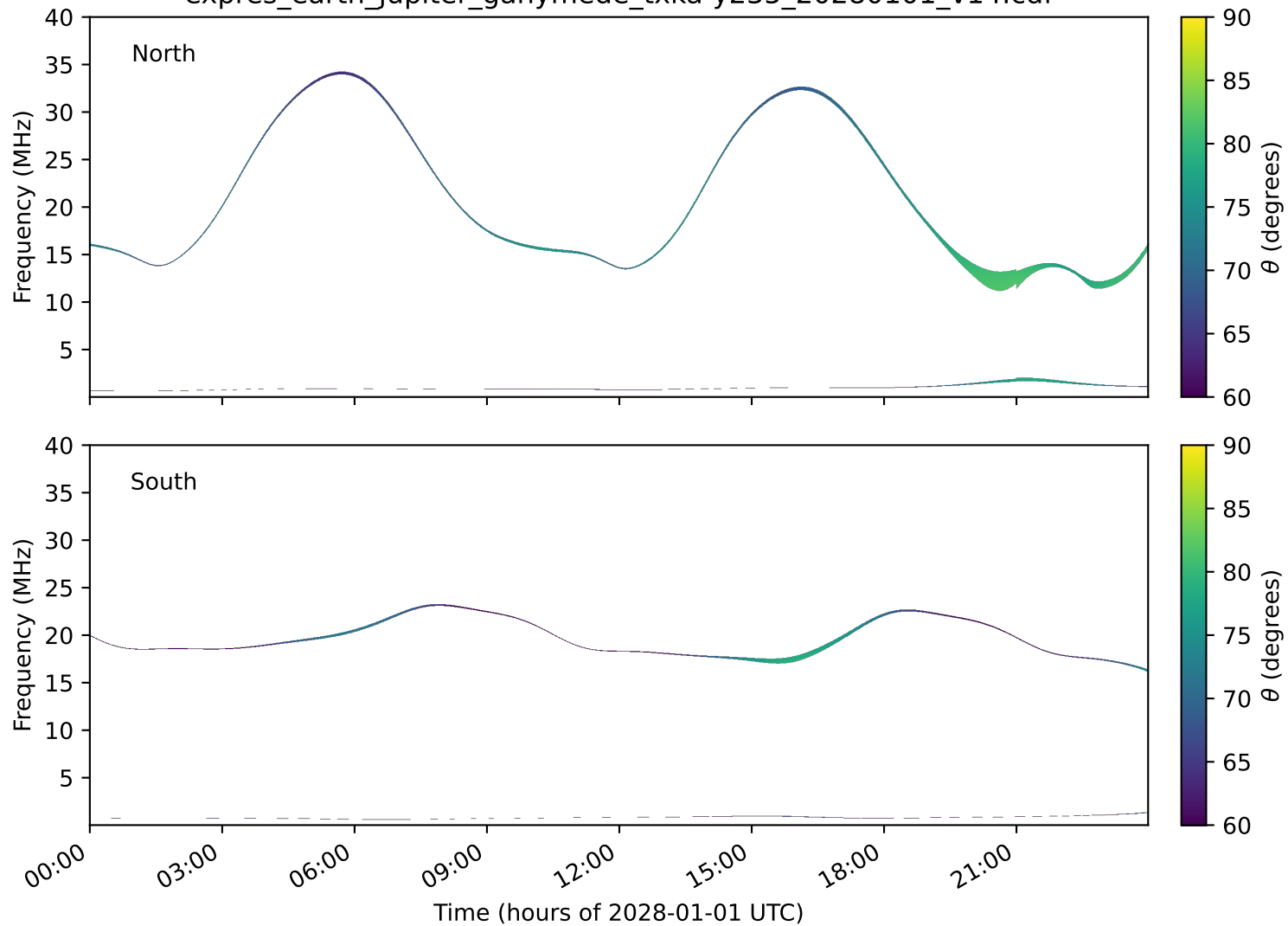
expres_earth_jupiter_ganymede_txka-y235_20280101_v14.cdf
