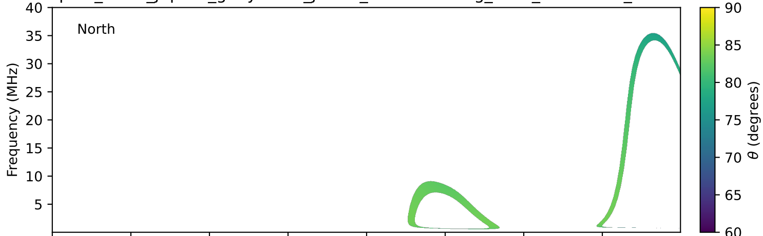
expres_earth_jupiter_ganymede_jrm33_lossc-wid1deg_3kev_20280106_v11.cdf
