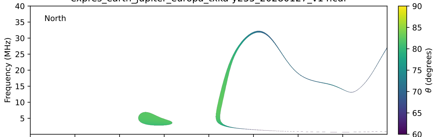
expres_earth_jupiter_europa_txka-y235_20280127_v14.cdf
