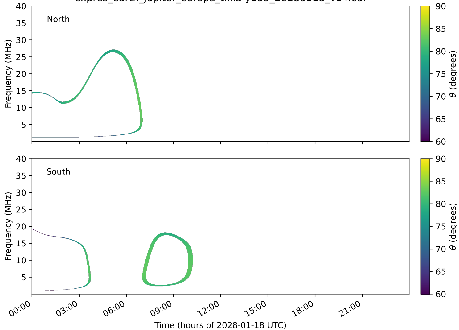
expres_earth_jupiter_europa_txka-y235_20280118_v14.cdf
