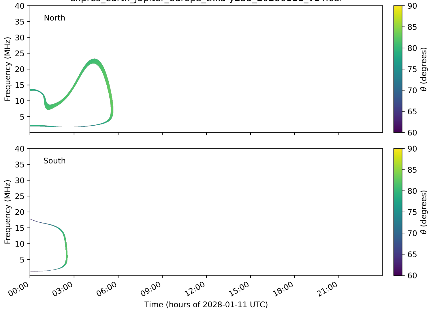
expres_earth_jupiter_europa_txka-y235_20280111_v14.cdf
