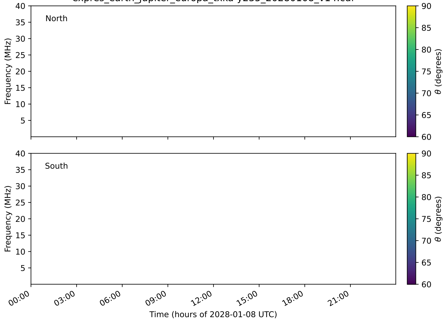
expres_earth_jupiter_europa_txka-y235_20280108_v14.cdf
