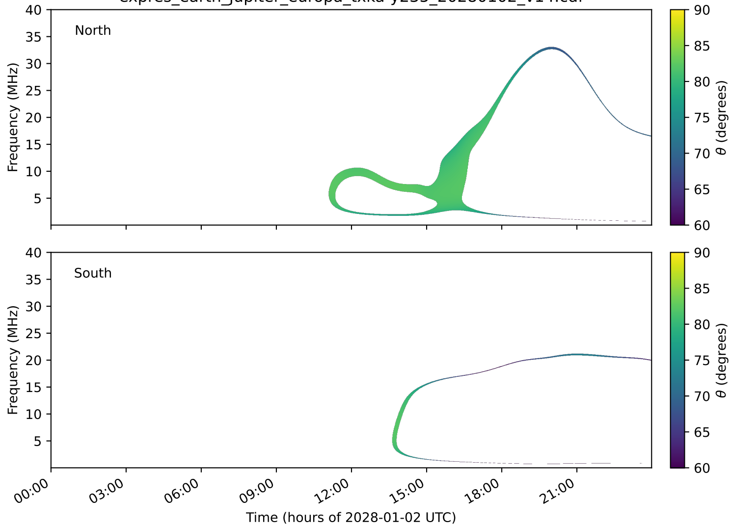
expres_earth_jupiter_europa_txka-y235_20280102_v14.cdf
