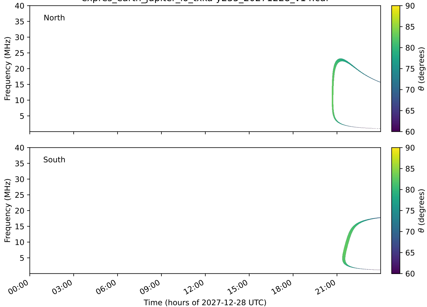
expres_earth_jupiter_io_txka-y235_20271228_v14.cdf
