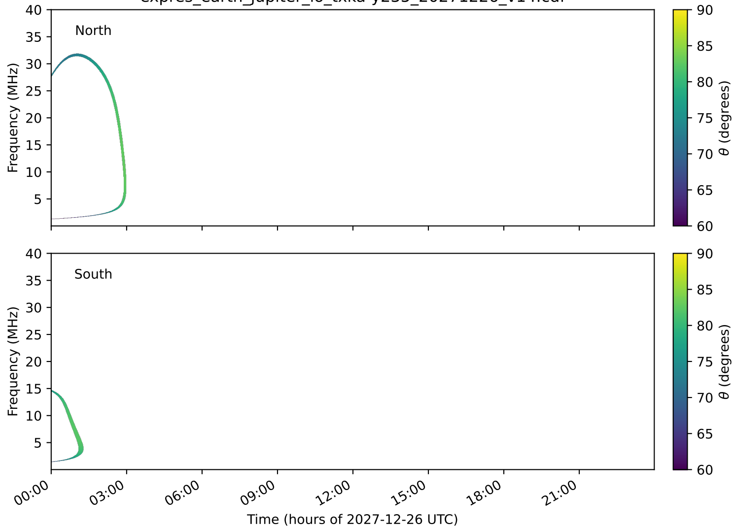
expres_earth_jupiter_io_txka-y235_20271226_v14.cdf
