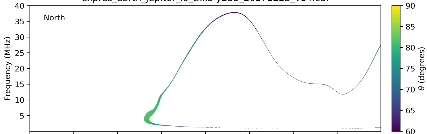
expres_earth_jupiter_io_txka-y235_20271225_v14.cdf
