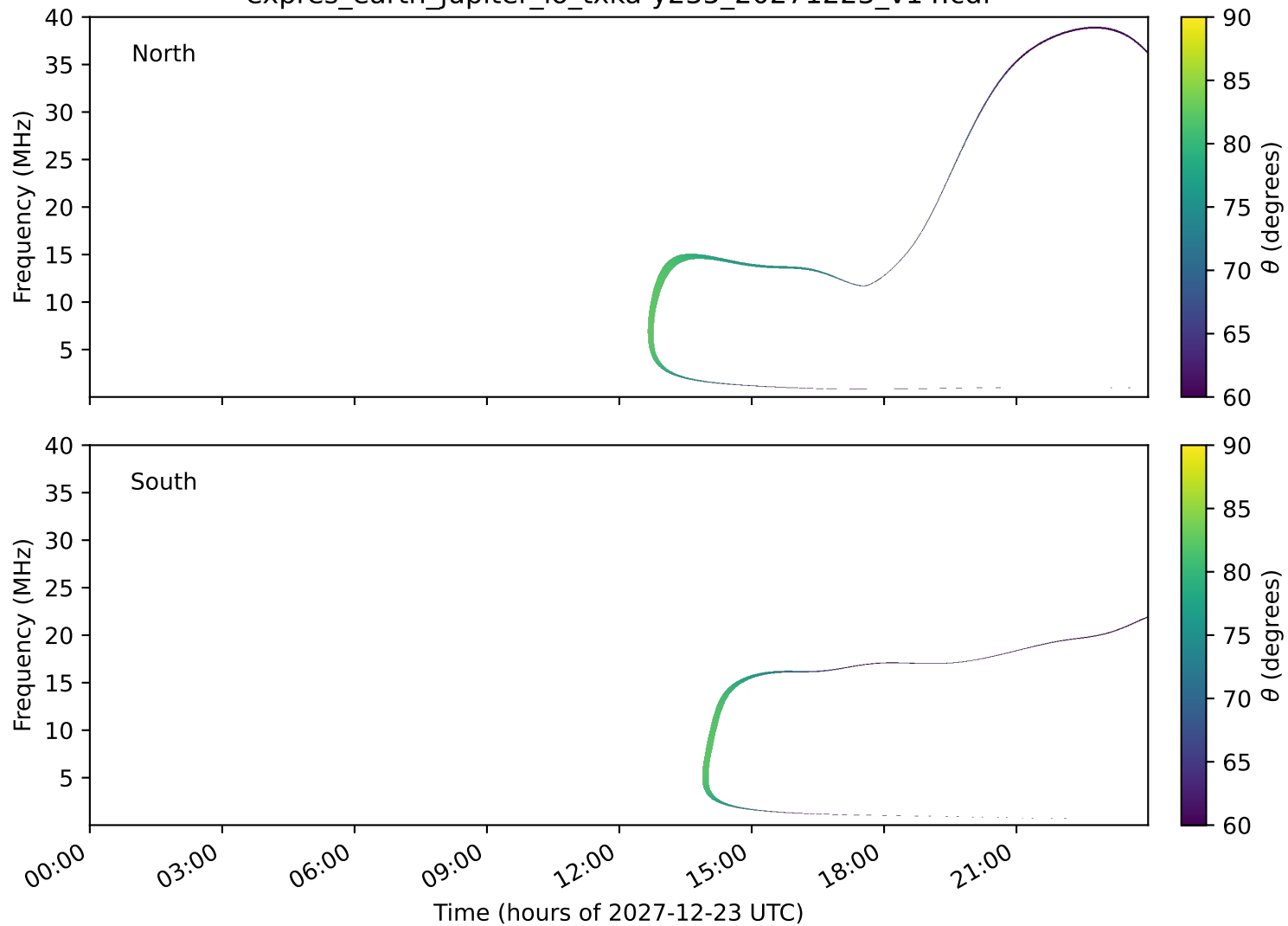
expres_earth_jupiter_io_txka-y235_20271223_v14.cdf
