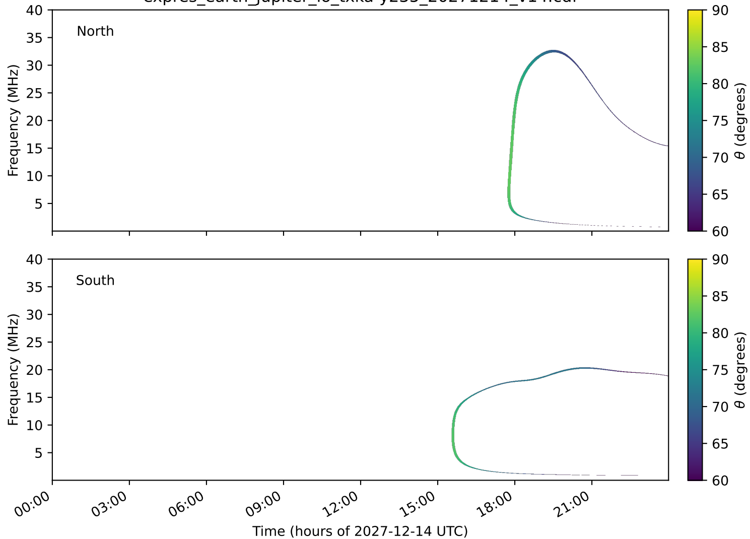
expres_earth_jupiter_io_txka-y235_20271214_v14.cdf
