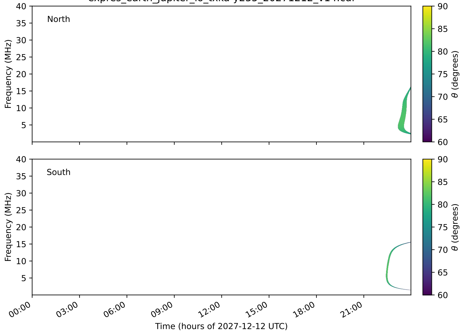
expres_earth_jupiter_io_txka-y235_20271212_v14.cdf
