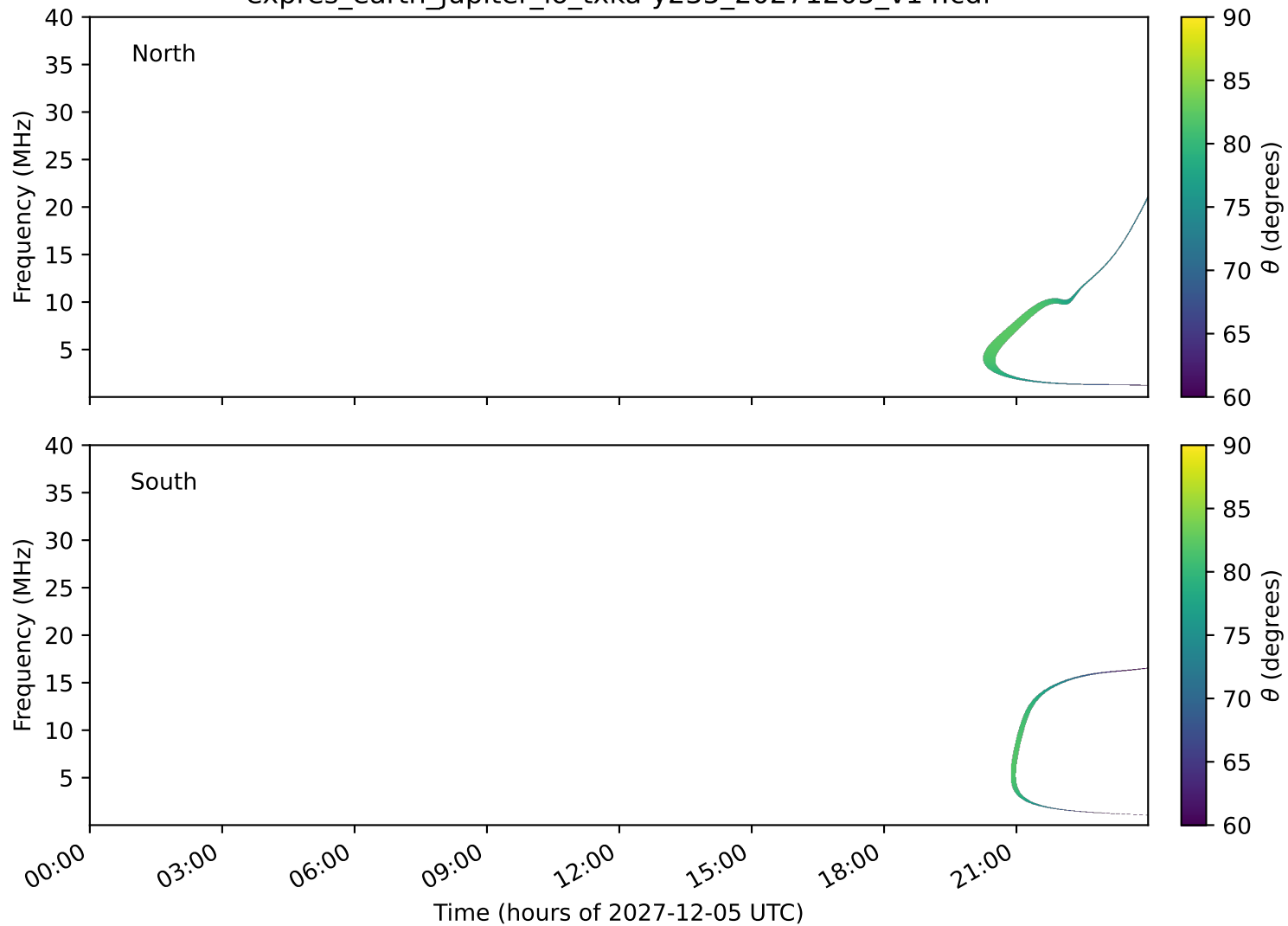
expres_earth_jupiter_io_txka-y235_20271205_v14.cdf
