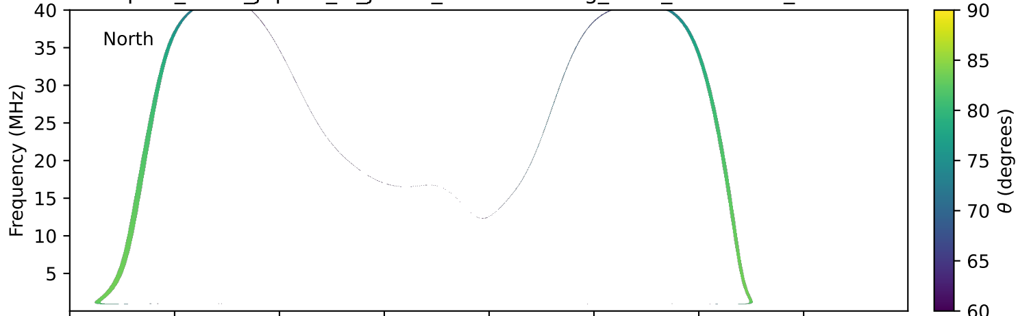
expres_earth_jupiter_io_jrm33_lossc-wid1deg_3kev_20271220_v11.cdf
