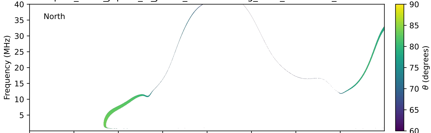
expres_earth_jupiter_io_jrm33_lossc-wid1deg_3kev_20271218_v11.cdf
