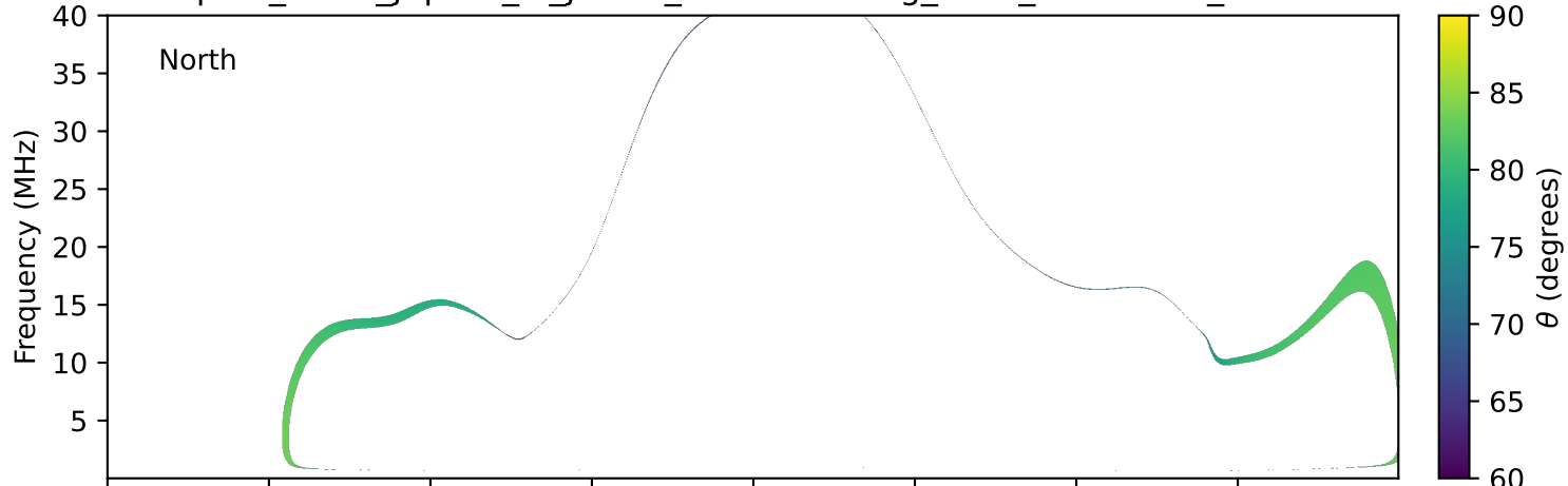
expres_earth_jupiter_io_jrm33_lossc-wid1deg_3kev_20271211_v11.cdf
