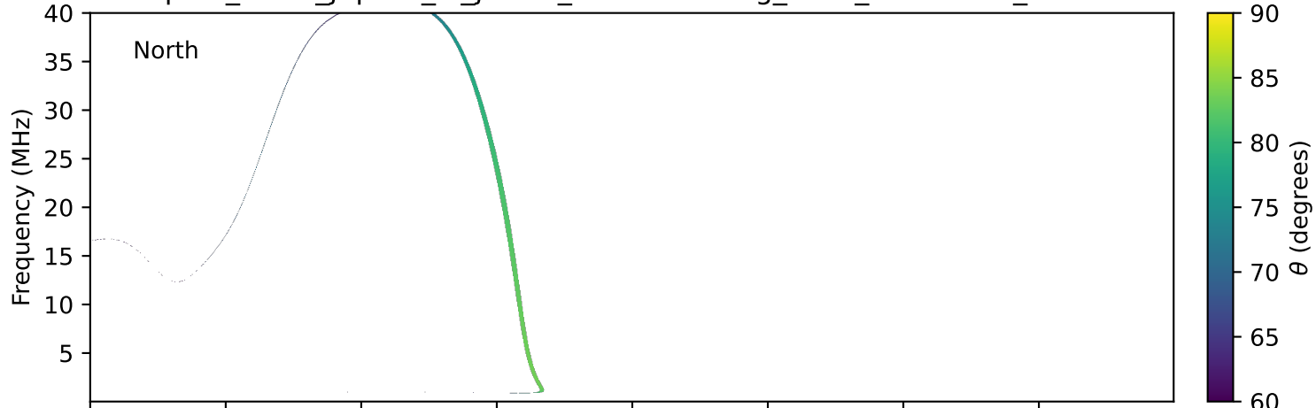
expres_earth_jupiter_io_jrm33_lossc-wid1deg_3kev_20271208_v11.cdf
