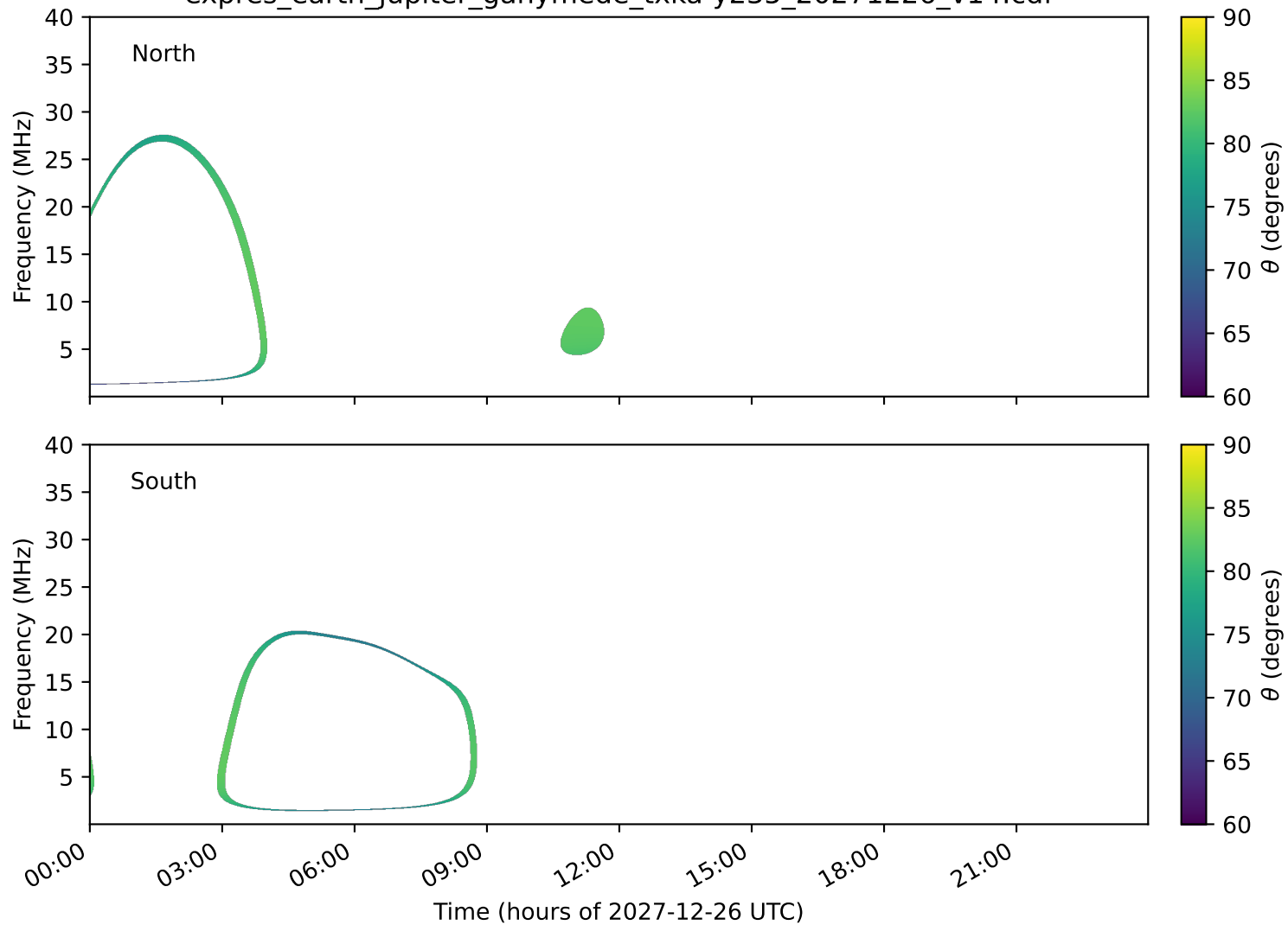
expres_earth_jupiter_ganymede_txka-y235_20271226_v14.cdf
