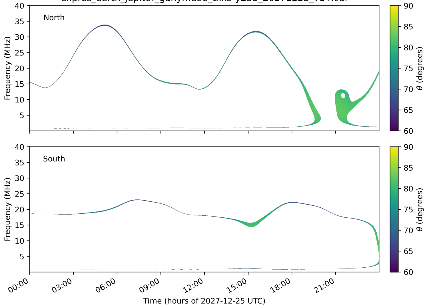
expres_earth_jupiter_ganymede_txka-y235_20271225_v14.cdf
