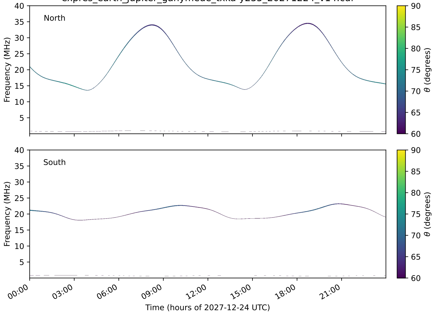
expres_earth_jupiter_ganymede_txka-y235_20271224_v14.cdf
