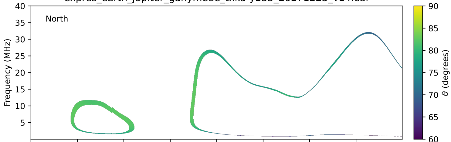
expres_earth_jupiter_ganymede_txka-y235_20271223_v14.cdf
