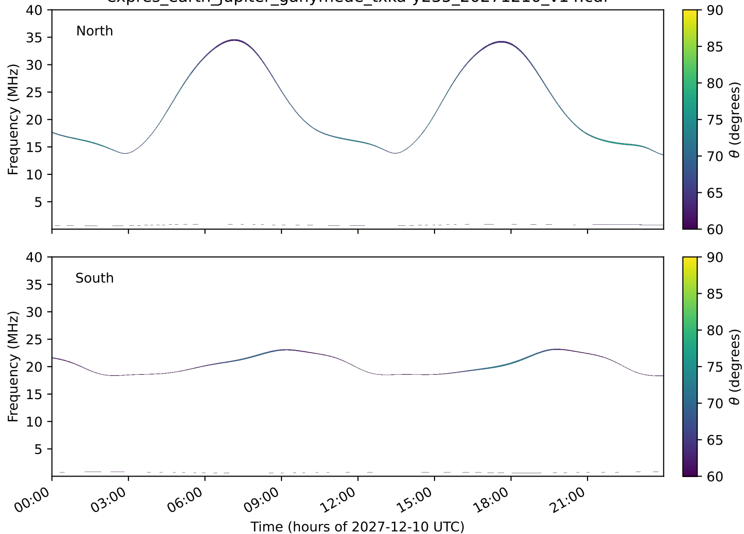
expres_earth_jupiter_ganymede_txka-y235_20271210_v14.cdf
