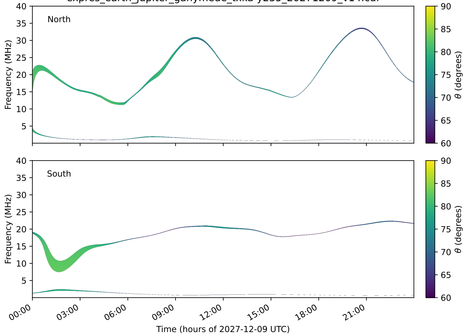
expres_earth_jupiter_ganymede_txka-y235_20271209_v14.cdf
