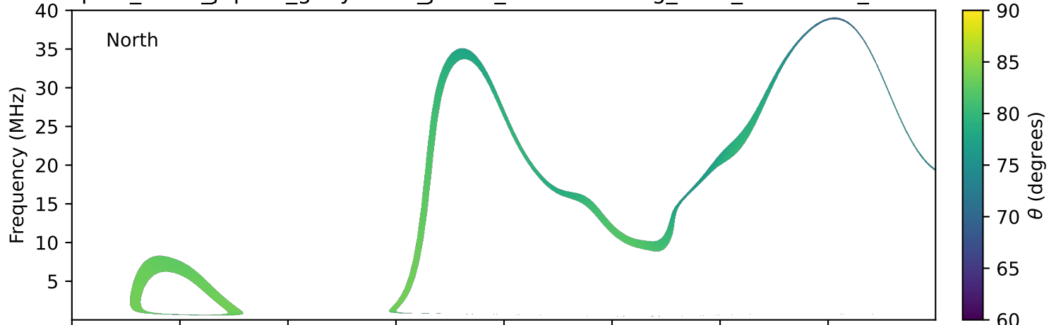
expres_earth_jupiter_ganymede_jrm33_lossc-wid1deg_3kev_20271216_v11.cdf
