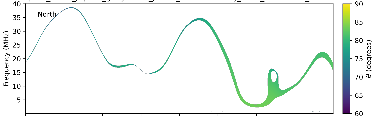
expres_earth_jupiter_ganymede_jrm33_lossc-wid1deg_3kev_20271204_v11.cdf
