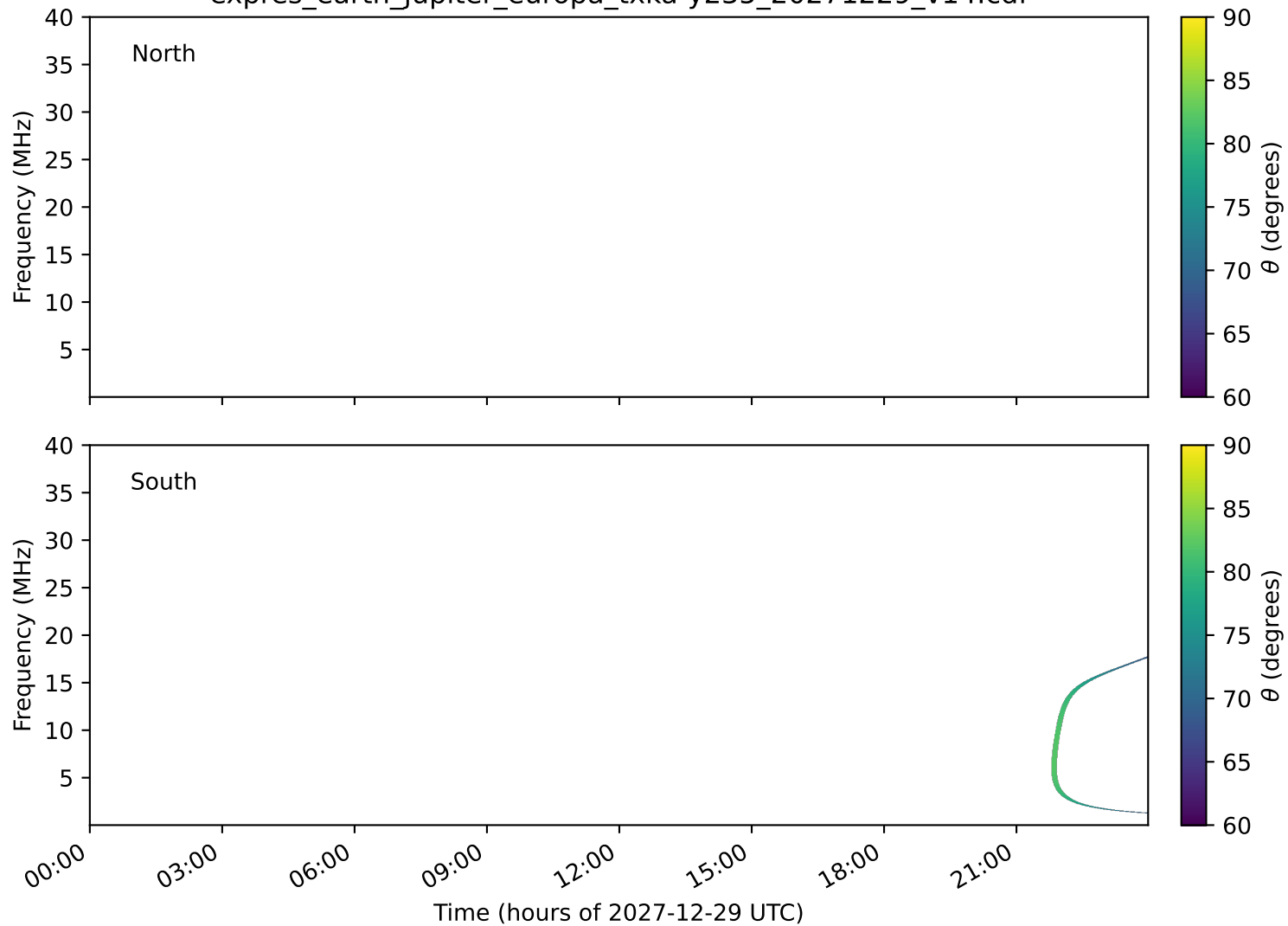
expres_earth_jupiter_europa_txka-y235_20271229_v14.cdf
