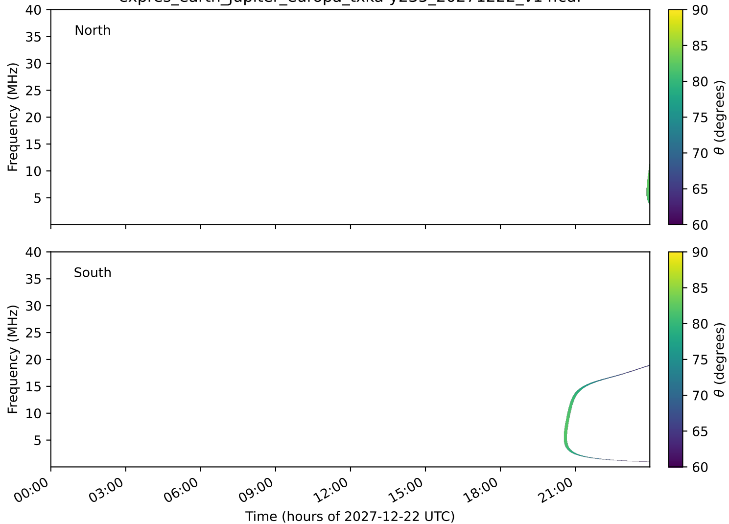
expres_earth_jupiter_europa_txka-y235_20271222_v14.cdf
