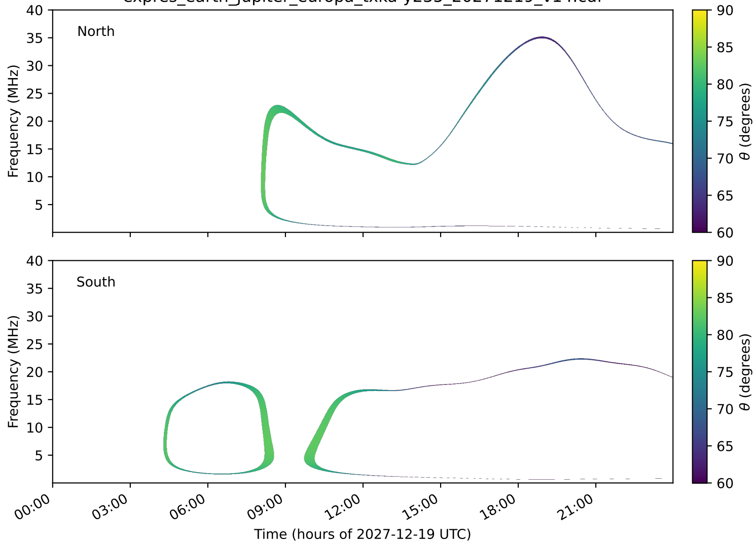
expres_earth_jupiter_europa_txka-y235_20271219_v14.cdf
