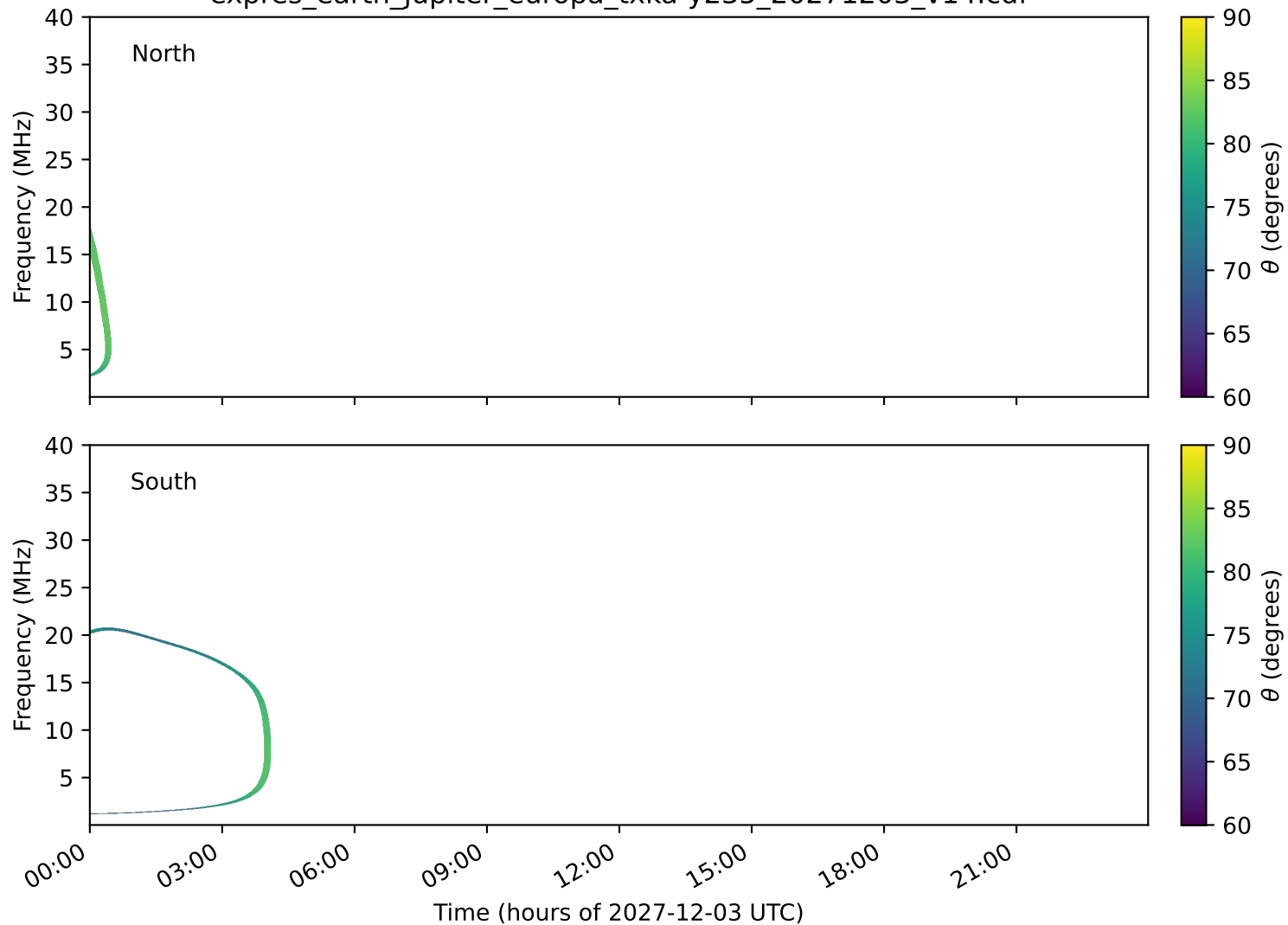
expres_earth_jupiter_europa_txka-y235_20271203_v14.cdf
