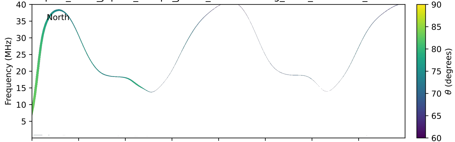
expres_earth_jupiter_europa_jrm33_lossc-wid1deg_3kev_20271223_v11.cdf
