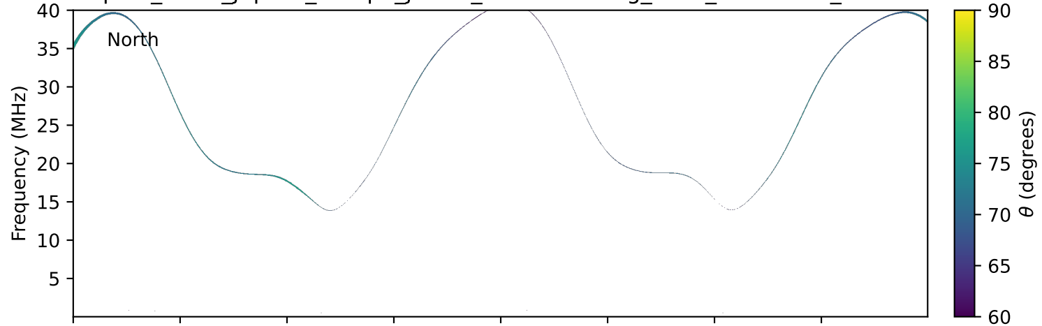
expres_earth_jupiter_europa_jrm33_lossc-wid1deg_3kev_20271216_v11.cdf
