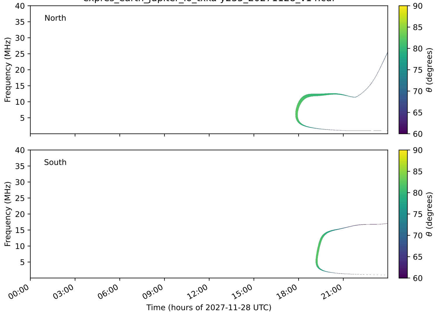
expres_earth_jupiter_io_txka-y235_20271128_v14.cdf
