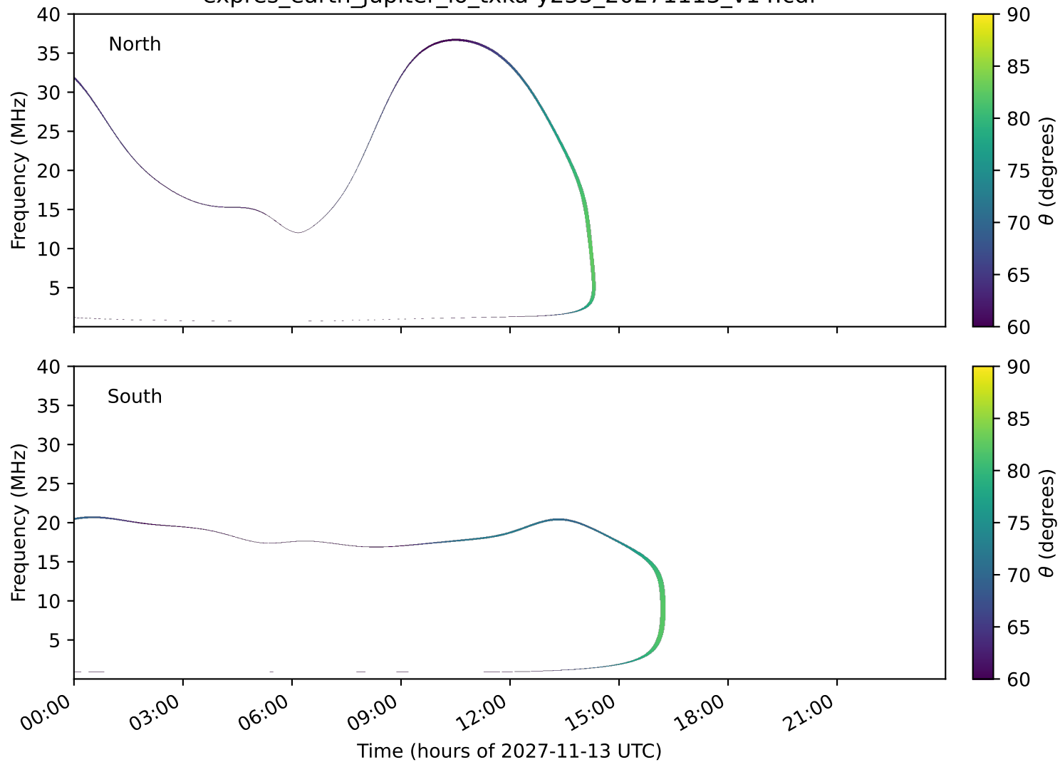
expres_earth_jupiter_io_txka-y235_20271113_v14.cdf
