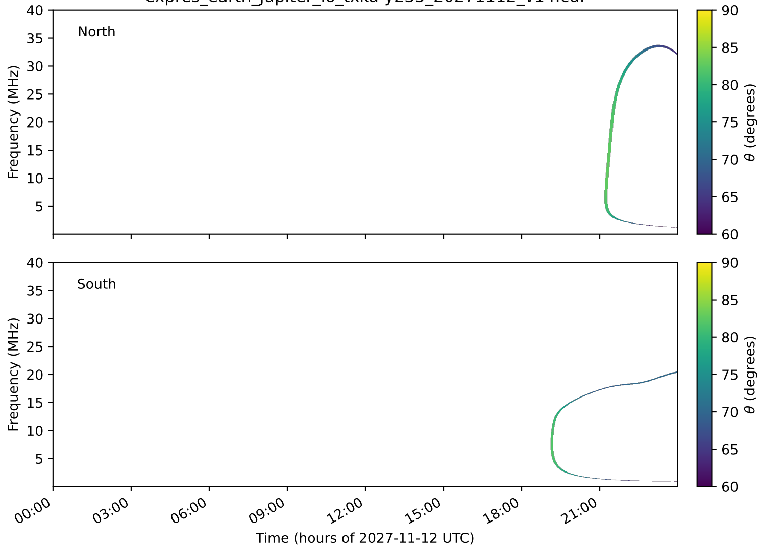
expres_earth_jupiter_io_txka-y235_20271112_v14.cdf
