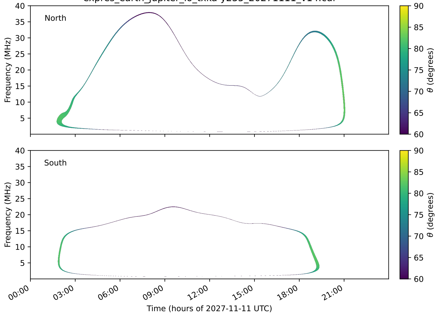
expres_earth_jupiter_io_txka-y235_20271111_v14.cdf
